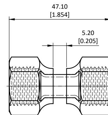
ASSEMBLY VIEW
