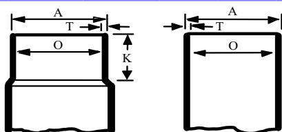
MALE (FITTING)
