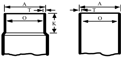
MALE (FITTING)
