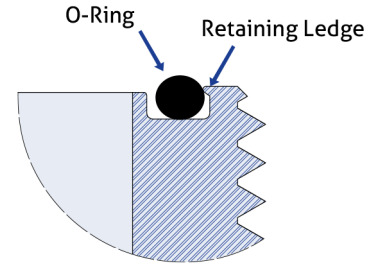
VIEW OF GROOVE TYPE B
