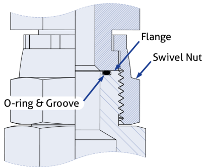
ORFS FITTING ASSEMBLY
