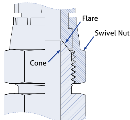
FLARE FITTING ASSEMBLY
